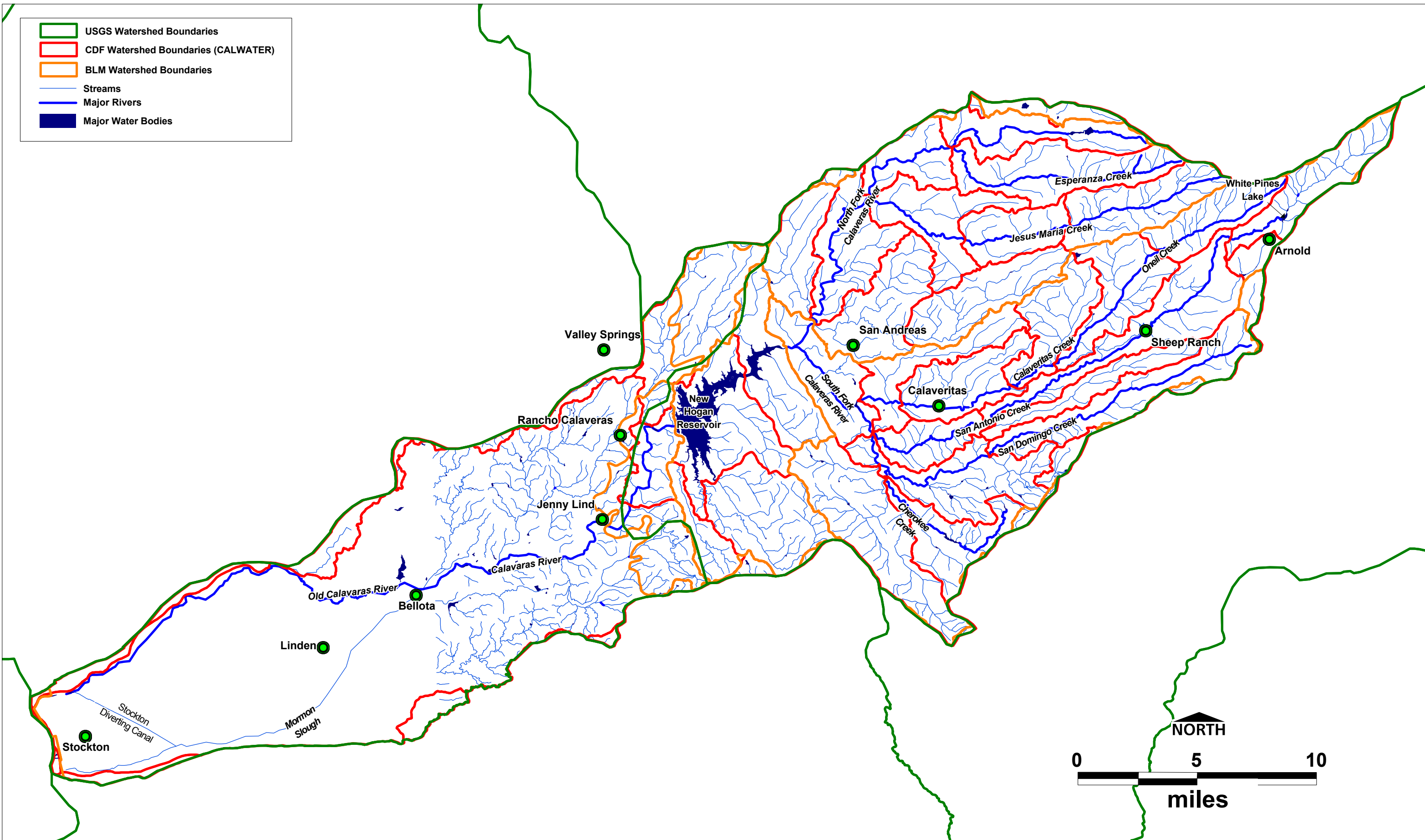
Figure 3-8. Planning Watersheds and Subwatersheds
