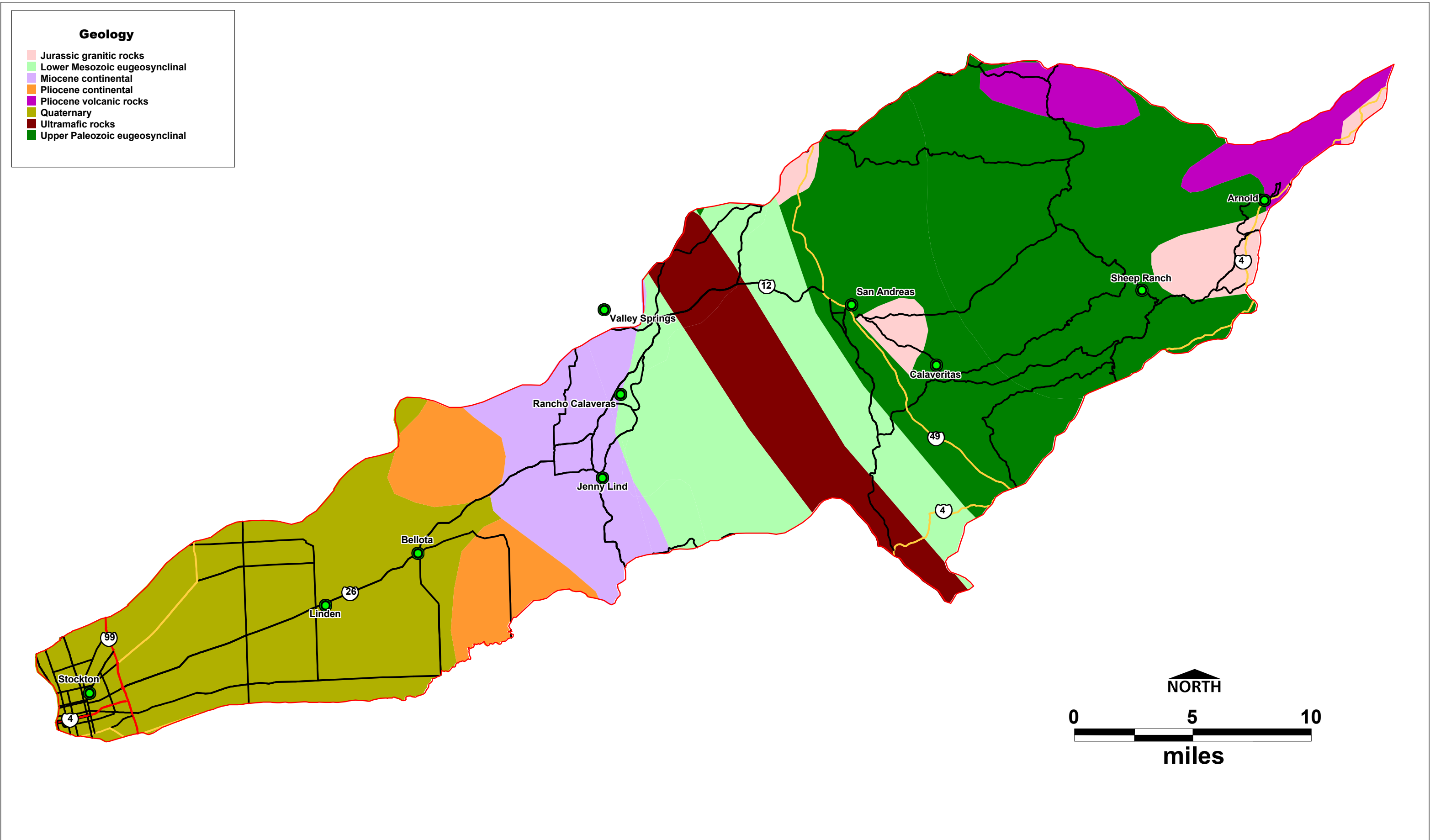
Figure 3-3. Conceptual Geology
